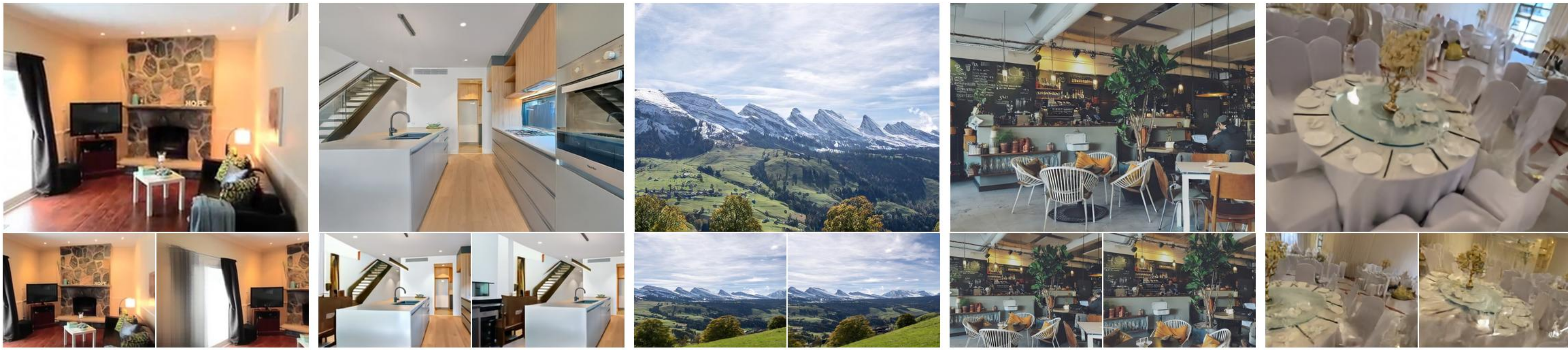
LVSM
