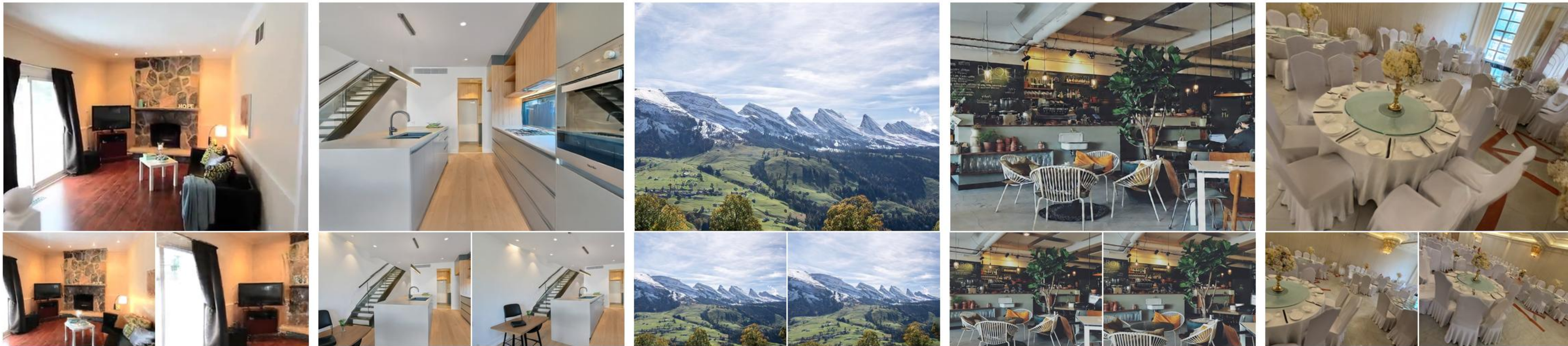
PixWorld (Ours)
