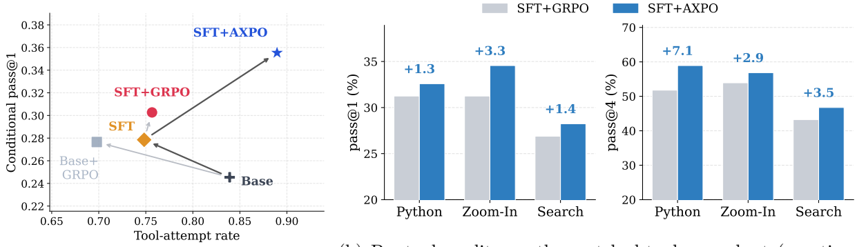
(a) Training stages on the tool-attempt rate vs. conditional pass@1 plane. Only AXPO improves pass@1 and pass@4 across all three tool families. (b) Per-tool quality on the matched-tool-use subset (questions where both SFT+GRPO and SFT+AXPO invoke the tool). AXPO improves Pass@1 across all three tool families, indicating the gain is in tool interaction quality.
