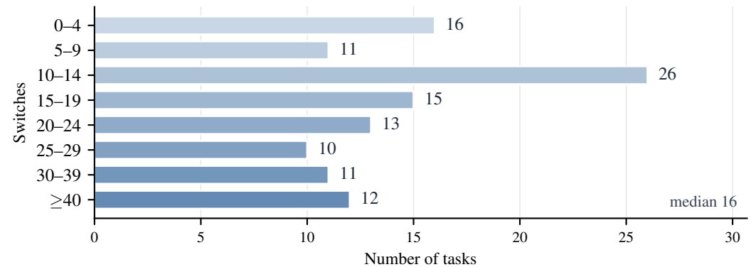
(b) GUI / CLI channel switches per task
