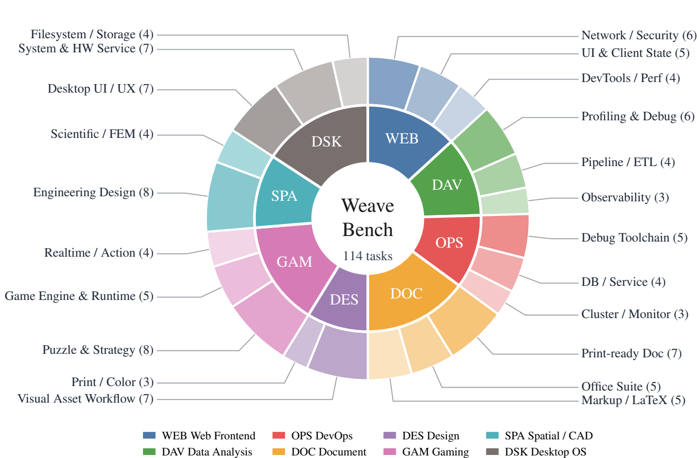
(a) Task taxonomy
