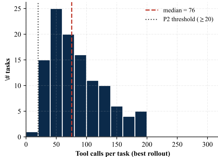
(a) P2: trajectory length median=76, mean=88; \geq 20 in 113/114 (99.1\%)
