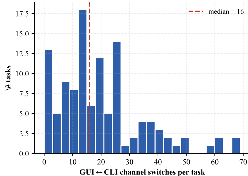
(b) GUI \leftrightarrow CLI switches median=16, mean=19.7; switch rate \approx 23\%
