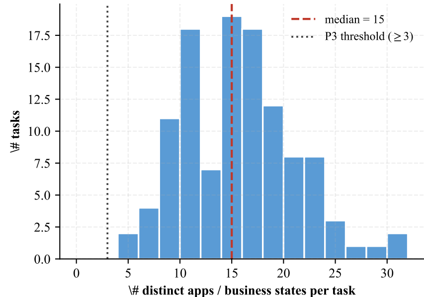
(c) P3: cross-application coverage median=15, mean=15.2; \geq 3 in 114/114 (100.0\%)
