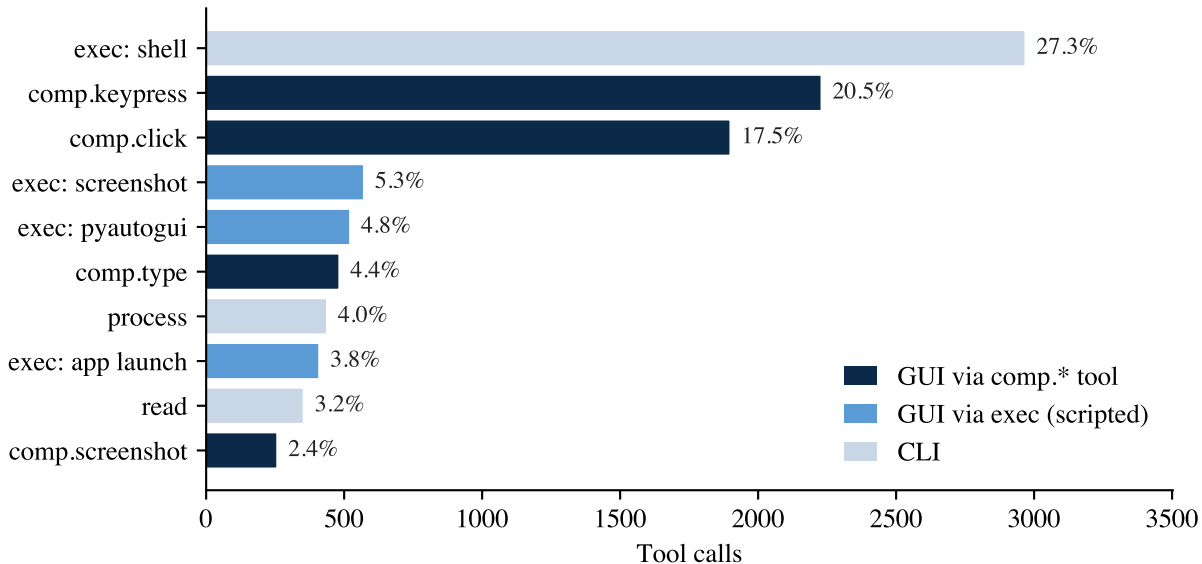
Top-10 atomic operations (GPT-5.5)
