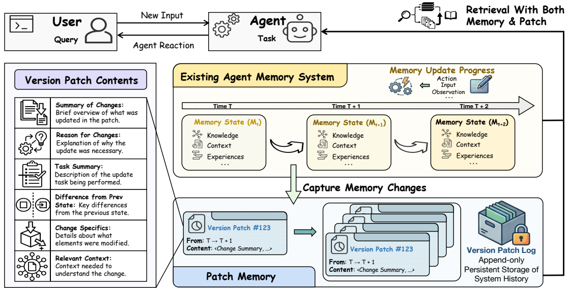
FIGURE 7 Overview of EvoMem. EvoMem augments a base memory system with an append-only patch history that records behaviorally meaningful memory updates and retrieves relevant patches as versioned evidence at inference time.
