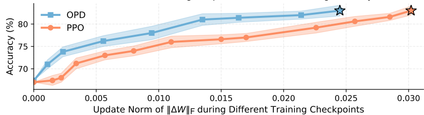
Qwen3-8B-Base PPO vs. OPD: Scaling of Update Norm vs. Reasoning Accuracy on MATH500
