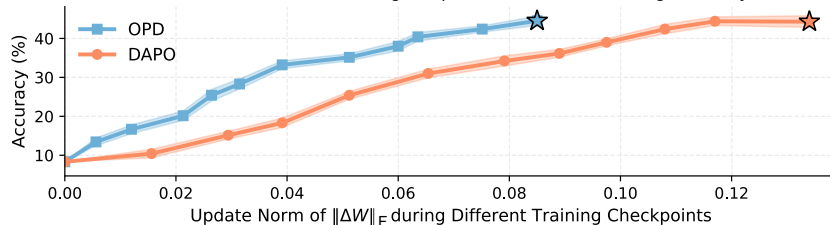
Qwen3-14B-Base DAPO vs. OPD: Scaling of Update Norm vs. Reasoning Accuracy on AIME26
