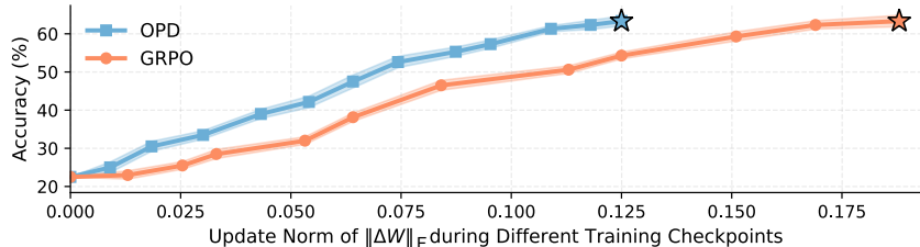
Qwen3-14B GRPO vs. OPD: Scaling of Update Norm vs. Reasoning Accuracy on AIME26
