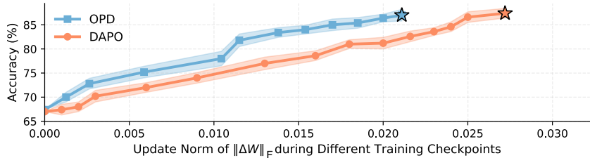
Qwen3-8B-Base DAPO vs. OPD: Scaling of Update Norm vs. Reasoning Accuracy on MATH500
