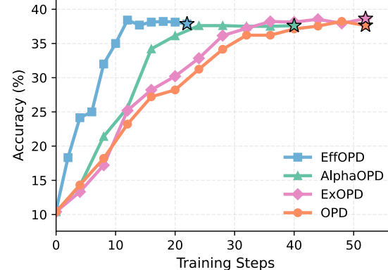
Qwen3-14B-Base on AIME25
