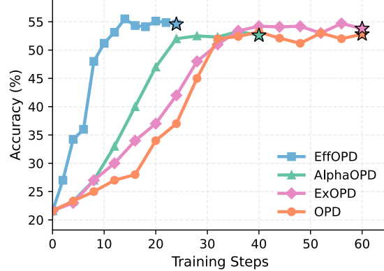
Qwen3-4B-Non-Thinking on AIME25
