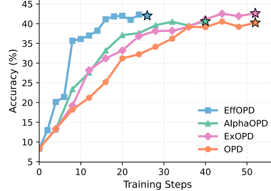
Qwen3-14B-Base on AIME26
