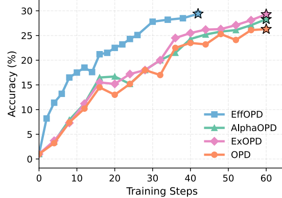
Qwen2.5-1.5B-Deepseek on Taco
