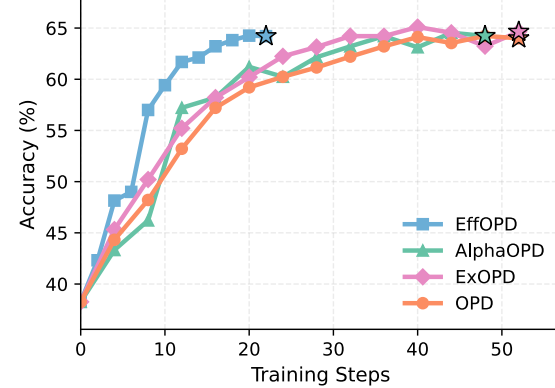
Qwen2.5-32B on GPQA
