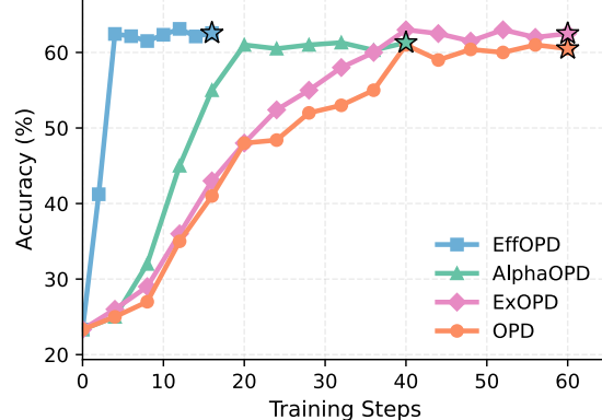
Qwen3-4B-Non-Thinking on AIME24
