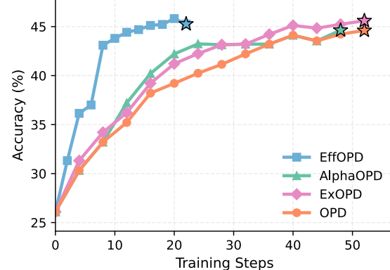
Qwen2.5-32B on MINERVA
