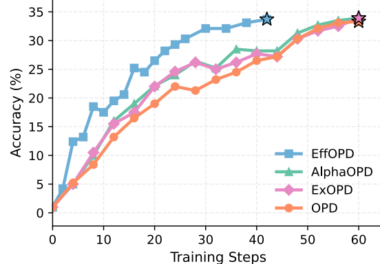
Qwen2.5-1.5B-Deepseek on Codeforces
