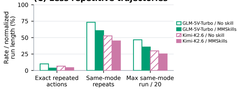
(C) Less repetitive trajectories
