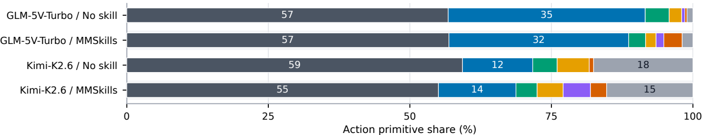
(B) Lower action load
