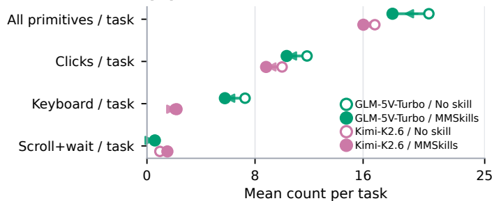
(B) Lower action load
