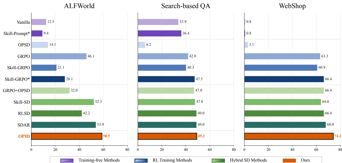
FIGURE 1 Overall performance comparison. We compare OPID with training-free prompting methods, outcome-only RL, and skill-distillation baselines on ALFWorld, Search-based QA, and WebShop. OPID achieves the strongest average performance on ALFWorld and WebShop while remaining competitive on Search-based QA.
