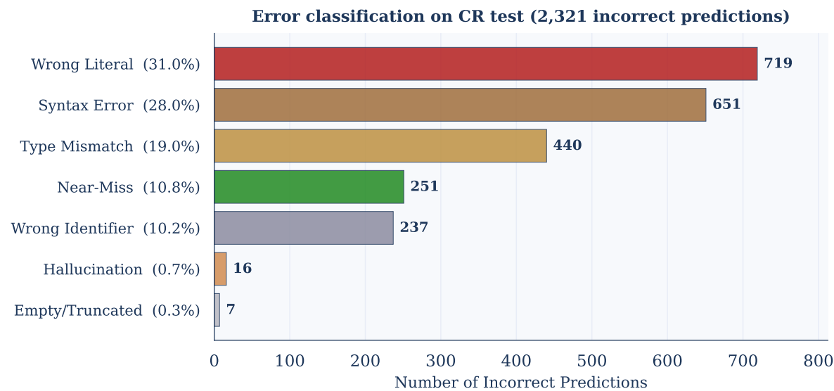
FIGURE 12 Error classification of Code2LoRA-Static failures on CR test (2,321 incorrect predictions), following a LiveCodeBench-inspired taxonomy. Wrong literal (31.0%), syntax error (28.0%), type mismatch (19.0%), near-miss (10.8%), wrong identifier (10.2%); hallucinations and empty outputs are < 1% each.
