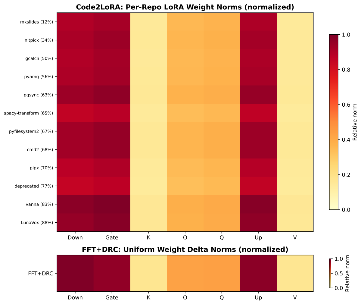
FIGURE 11 Comparison of per-module weight norms. Top: Code2LoRA-Static generates repo-specific LoRA adapters with varying weight distributions across module types. Bottom: FFT+DRC applies a uniform weight delta. Code2LoRA-Static’s structured, repo-specific adaptations explain its stronger cross-repo performance.
