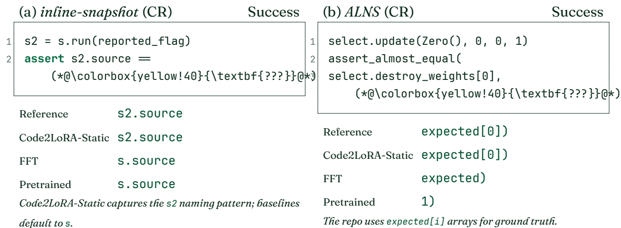
FIGURE 13 Qualitative examples from CR test. Each panel shows a test prefix with the completion target ( ??? ), ground-truth reference, and model predictions. (a)–(b): Code2LoRA-Static correctly infers repo-specific identifiers and conventions that pretrained Qwen2.5-Coder and full fine-tuning miss.
