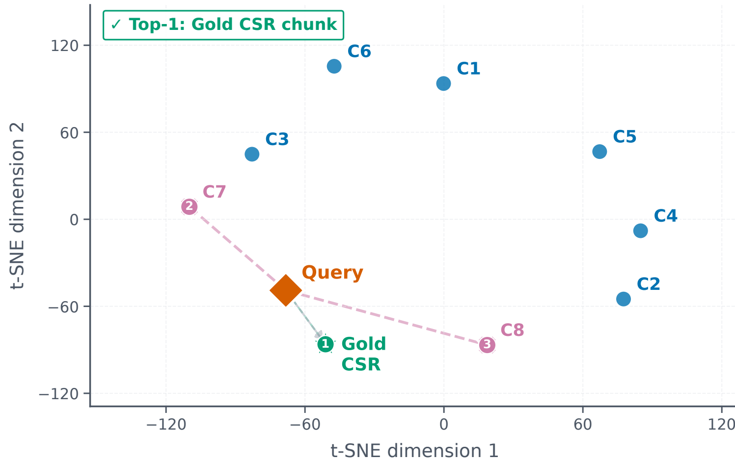
(a) Raw Embedding Space
