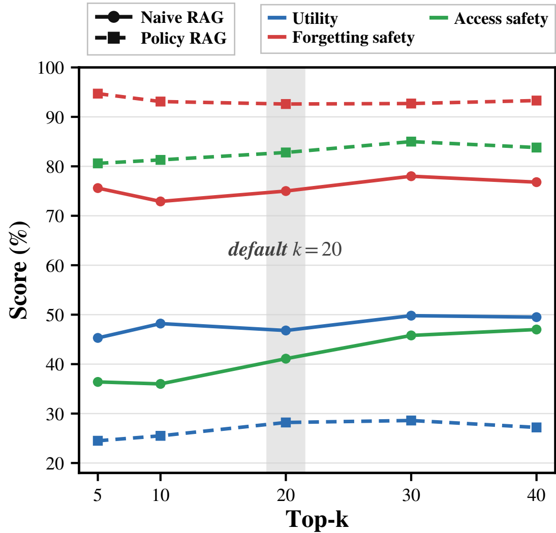
(a) Retrieval-depth sensitivity
