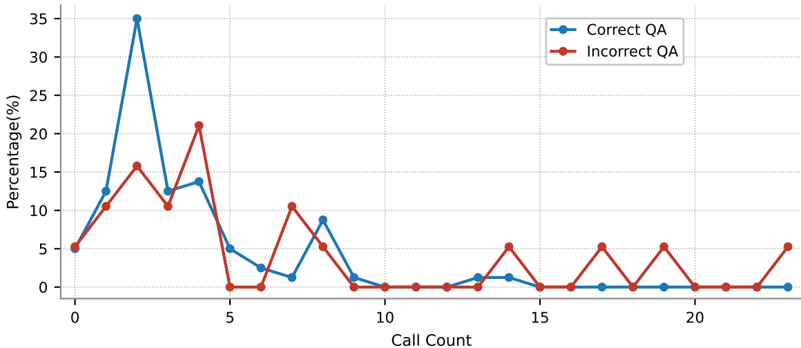
xbench-DeepSearch-2505 - Main Calls To Sub-Agents Acc: 80.8%
