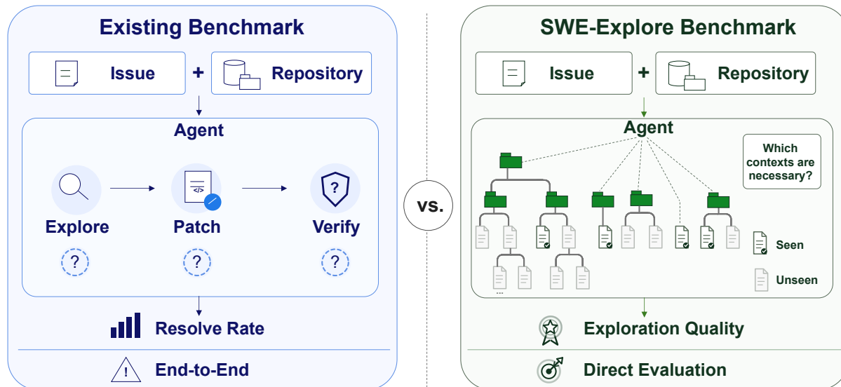
FIGURE 1 Motivation of SWE-Explore. A holistic metric of resolution rate conflates exploration, localization, and patch synthesis. SWE-Explore isolates repository exploration as a line-level evaluation target.
