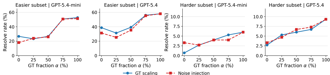
FIGURE 5 Resolve rate as the visible context degrades from the Oracle’s full core set R_{\text{core}} to either \alpha\% of R_{\text{core}} alone ( GT scaling , solid) or \alpha\% of R_{\text{core}} padded back to full size with random non-core regions ( noise injection , dashed).
