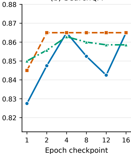
(b) SearchQA
