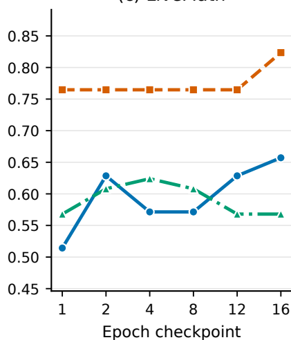
(c) LiveMath
