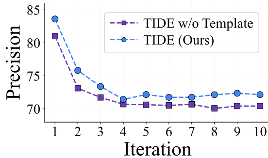
FIGURE 6 Per-iteration retrieval coverage (left) and precision (right) on the Workspace setting with GPT.
