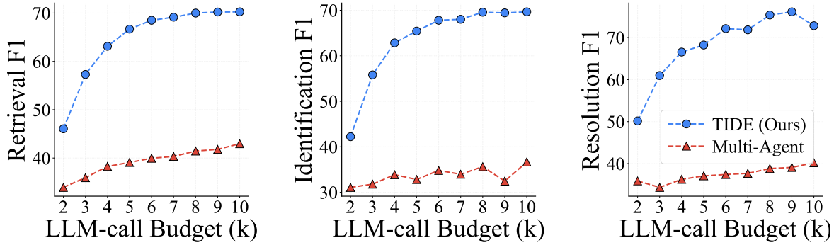
FIGURE 4 F1 results as a function of the per-instance LLM-call budget k on the Workspace setting with GPT.
