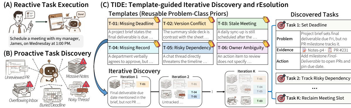
FIGURE 1 Conceptual illustration of TIDE. (A) Reactive agents act only on explicit user requests, leaving (B) the many problems coexisting hidden across the user context untouched. (C) TIDE surfaces them by applying reusable thought templates over multiple rounds of iterative discovery conditioned on the cumulative state, returning per-task plans that identify, ground, and resolve each discovered problem.
