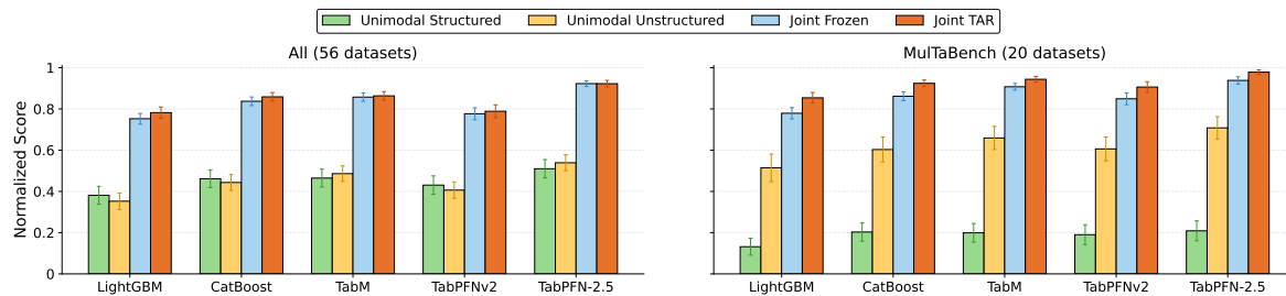
FIGURE 8 Curations Conditions for the Text-Tabular Pool. Normalized scores for Structured , Unstructured , Joint Frozen , and Joint TAR across all 56 candidates (left) and the MulTaBench subset (right).
