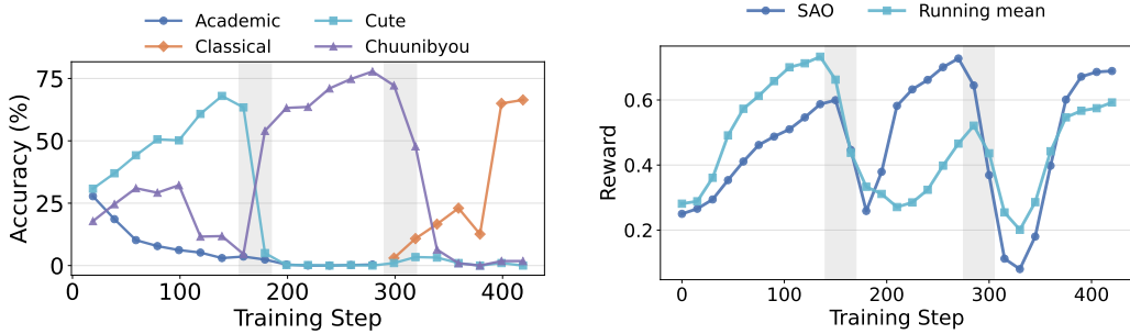
(a) We report the accuracy transition of three writing styles—cute, chuunibyuu, and classical—on a held-out evaluation set throughout the online training process. Shaded regions indicate phase transitions where the reward preference is switched to favor a different stylistic archetype. SAO rapidly suppresses the previously dominant style and realigns its policy to the new target based on environmental feedback. (b) We compare the evolution of training rewards between SAO and a Running Mean Advantage Estimation baseline under single-rollout online learning. Shaded regions denote stylistic reward shifts. While both methods eventually recover after distribution changes, the Running Mean baseline exhibits a pronounced adaptation lag and lower stable performance.
