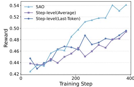
Figure 6: Training reward for token-level SAO training and step-level variants, where token-level shows better training rewards.
