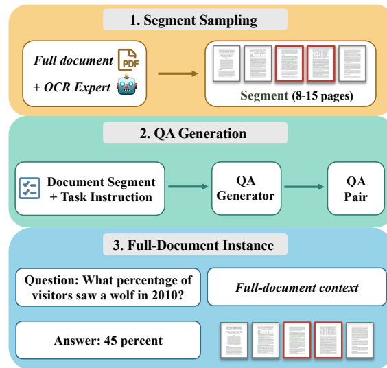
FIGURE 1 Long-document VQA synthesis pipeline. We first parse the full document with an OCR expert and sample a coherent segment. An LLM used as a QA generator (e.g., Seed 2.0) then produces a QA pair from the segment, which is inserted back into the original document to form a long-context training instance.
