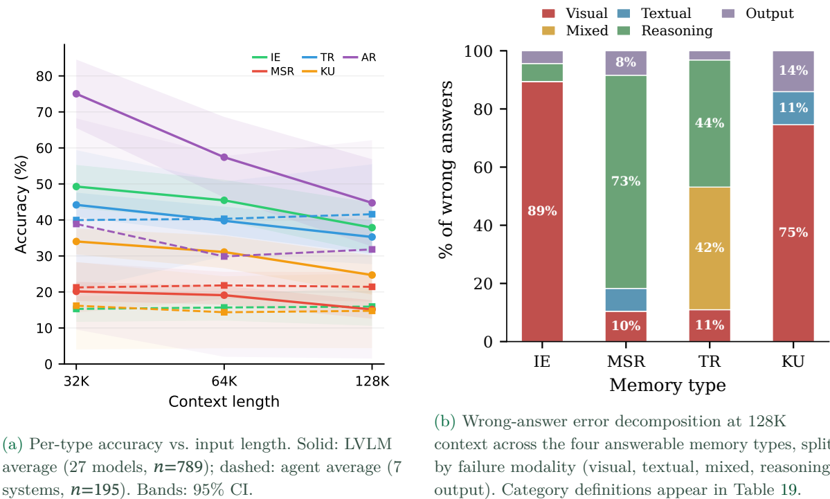
FIGURE3 Memory-ability specialization across representative LVLMs and memory agents.
