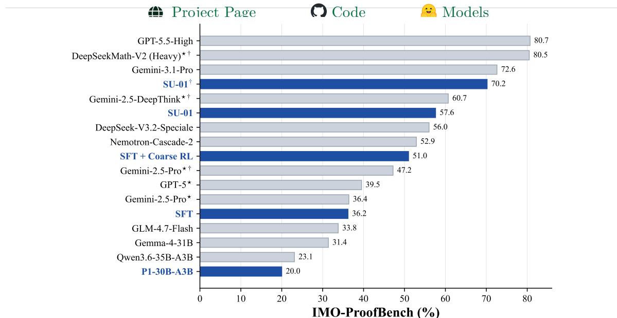
FIGURE 1 Overall comparison on IMO-ProofBench. ★ denotes results reported in the original paper, and † denotes results with test-time scaling. Blue bars trace the evolution of our pipeline from the 30B-A3B backbone through rigorous SFT (Section 2), coarse RL, refined RL (Section 3), and test-time scaling (Section 4), culminating in gold-medal-level olympiad reasoning (Section 5).
