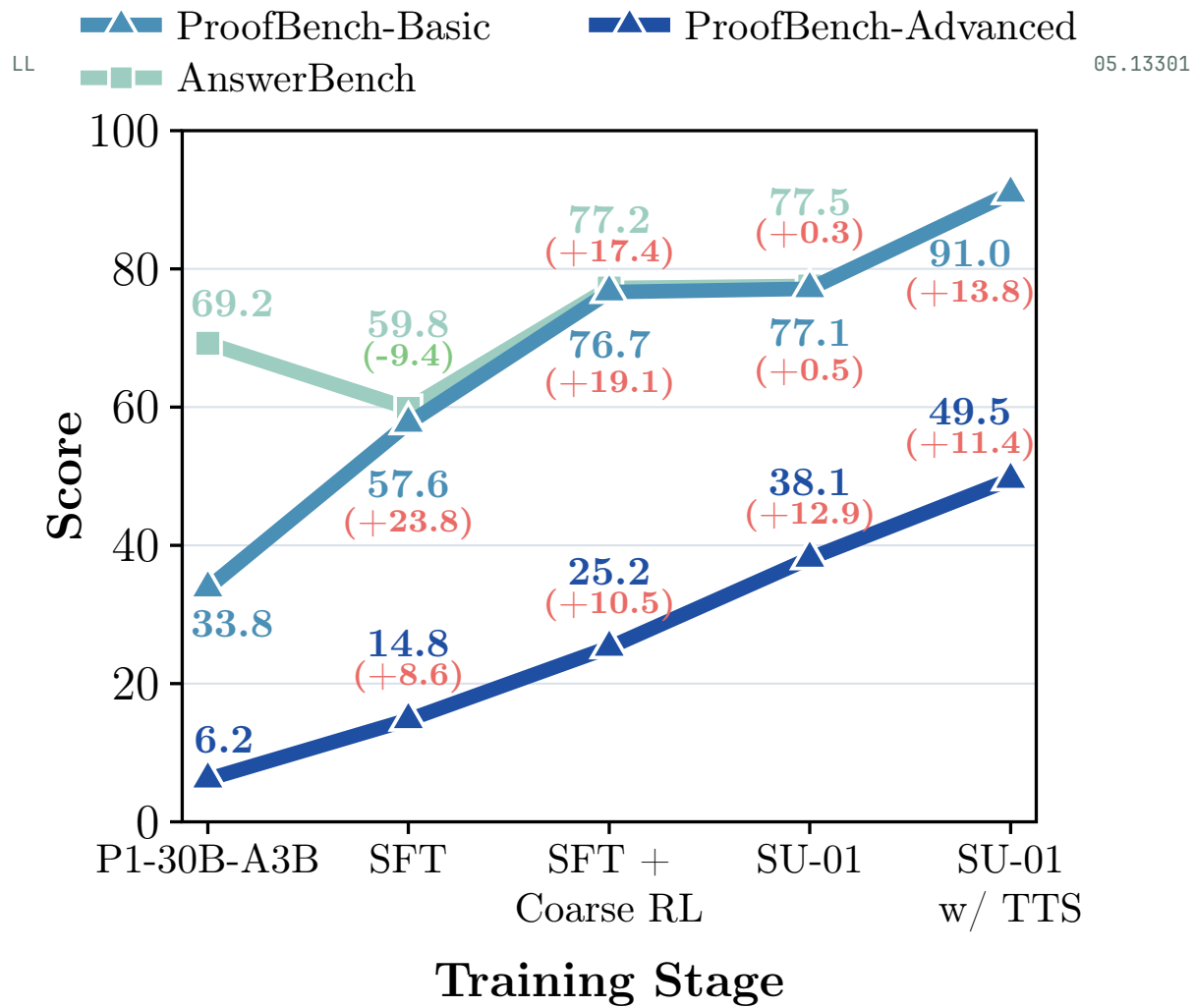
FIGURE 4 Progressive reasoning performance across training stages.
