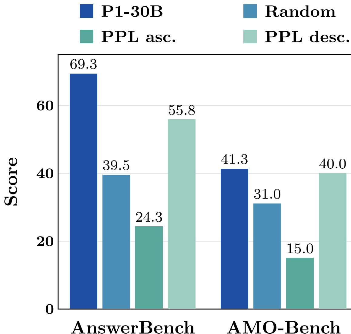
FIGURE 6 Validation results for SFT data ordering.
