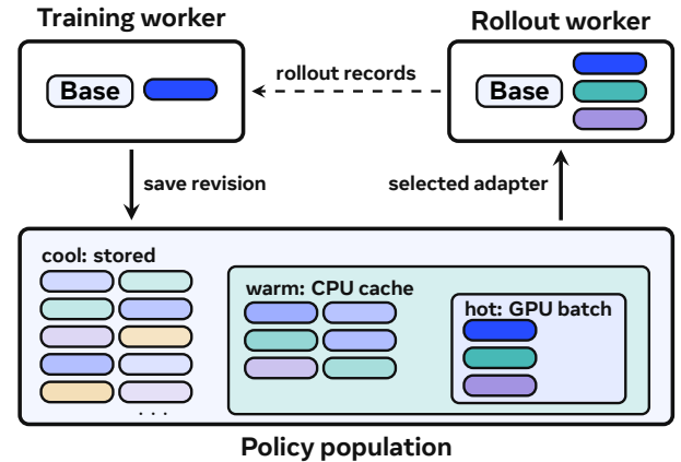
Figure 3 Adapter lifecycle in MinT. Training saves revisions into the policy population; rollout uses the hot GPU-batch subset and returns records for the next update.
