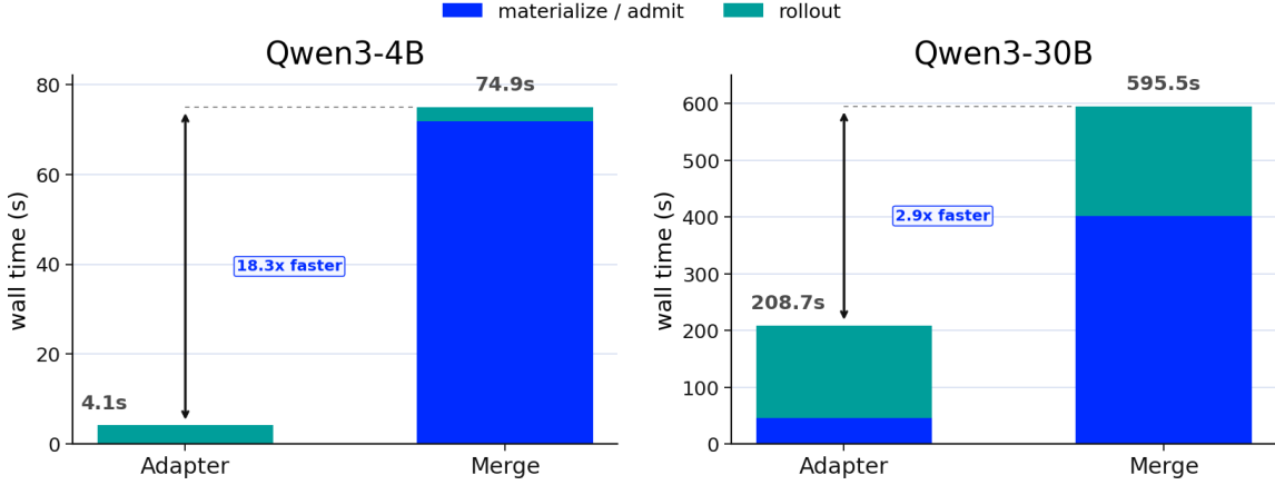
Figure 7 Adapter handoff avoids the merge-and-load stages that dominate the full-checkpoint path. Each stacked bar separates materialization or adapter loading from rollout under the probe protocol for the corresponding model.
