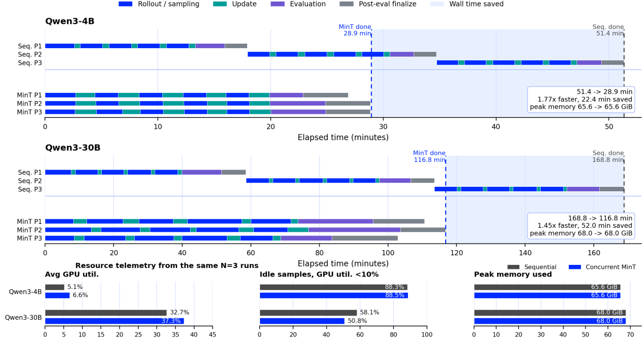
Figure 8 Concurrent multi-LoRA training overlaps GRPO runs under the same base-model allocation. Timeline lanes show the schedule, and the lower panels summarize average GPU utilization, samples below 10% utilization, and peak memory from the same runs. Vertical dashed lines mark completion time for the concurrent and sequential schedules.
