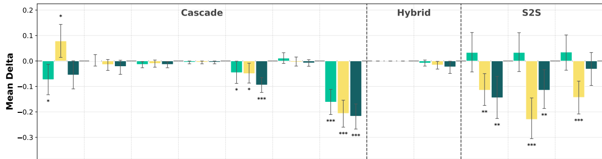
FIGURE9 Perturbation effect on EVA-X pass@1 across all evaluated systems, pooled across the three EVA domains. Bars show the mean delta from clean trials (negative = drop under perturbation); whiskers are 95% percentile bootstrap CIs on the per-scenario delta. Bar colors encode the perturbation condition: ■ accent, ■ background noise, ■ accent + background noise. Asterisks mark cells significant after Holm-Bonferroni correction within each model (* p < 0.05 , ** p < 0.01 , *** p < 0.001 ). Models, left to right: Cascade : Cohere + Gemma-4-26B + Voxtral, ElevenAgents (Scribe + Gemini-3-Flash + Conversational v3), Ink + Haiku-4.5 + Sonic, Nova + GPT-5.4 + Sonic, Nova + GPT-5.4-mini + Aura, Parakeet + Gemma-4-31B + Kokoro, Whisper + Qwen3.5-27B + Voxtral; Hybrid : Gemini-3-Flash + Gemini-3.1-Flash, Ultravox; S2S : Gemini-3.1-Flash-Live, GPT-Realtime-1.5, GPT-Realtime-mini.
