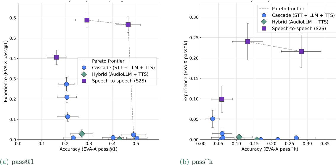
FIGURE 2 Accuracy vs Experience overview. Accuracy and Experience scores for pass@1 and pass k , mean \pm 95% CIs across domains. On the pass@1 plot, four systems are on the Pareto frontier, two S2S and two cascade: Gemini-3.1-Flash-Live, GPT-Realtime-1.5, Scribe + Gemini-3-Flash + Conversational v3, and Nova + GPT-5.4 + Sonic (left to right). On the pass k plot, only the two S2S systems are on the frontier (note axis range differences).
