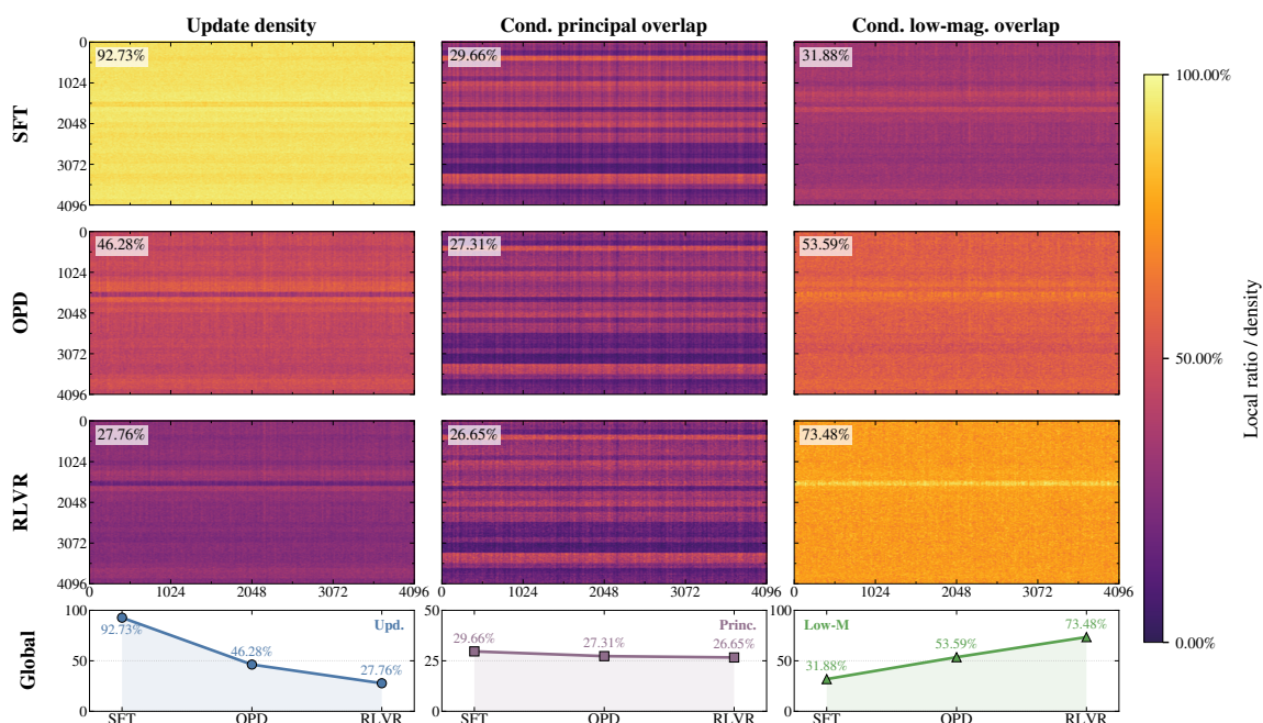
FIGURE3 Update-mask localization. We compare where bf16-visible updates land relative to principal and low-magnitude masks. OPD shifts updates away from principal weights and toward low-magnitude regions, while remaining less selective than RLVR.
