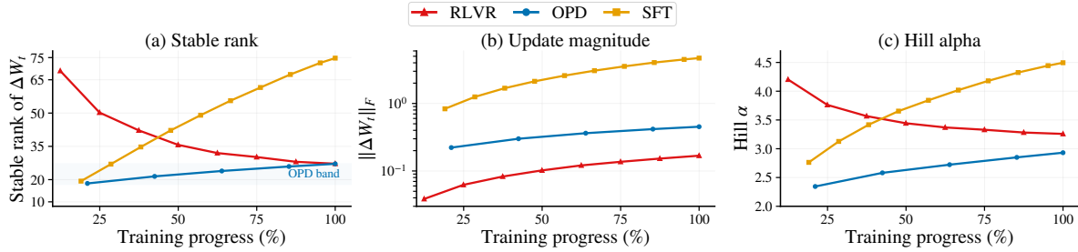
FIGURE 4 Intrinsic update geometry. We track cumulative updates \Delta W_t . OPD stays in a narrow stable-rank band, whereas SFT expands and RLVR contracts. Frobenius norms rule out a small-update explanation: OPD moves more than RLVR while ending with comparable stable rank. Hill estimates provide an auxiliary spectral-shape check.
