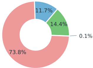
BrowseComp
