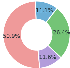
GAIA
