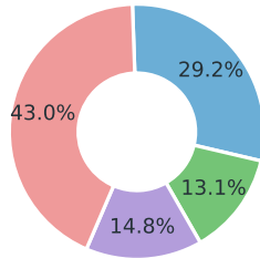
xbench
