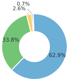
BrowseComp
