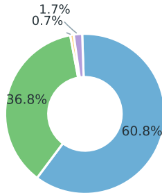
xbench
