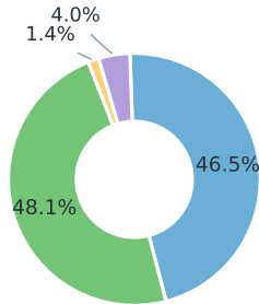
GAIA
