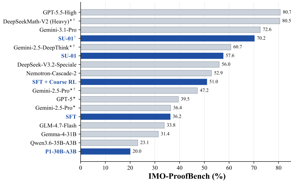
FIGURE 1 Overall comparison on IMO-ProofBench. ★ denotes results reported in the original paper, and † denotes results with test-time scaling. Blue bars trace the evolution of our pipeline from the 30B-A3B backbone through rigorous SFT (Section 2), coarse RL, refined RL (Section 3), and test-time scaling (Section 4), culminating in gold-medal-level olympiad reasoning (Section 5).
