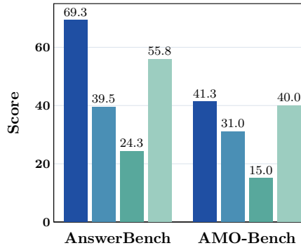
FIGURE 6 Validation results for SFT data ordering.
