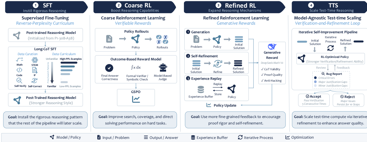
FIGURE 2 Overview of the SU-01 training and inference pipeline. The recipe first reshapes the backbone with rigorous long-form SFT, then scales the resulting behavior through coarse and refined RL, and finally applies test-time verification and refinement for olympiad-level problem solving.
