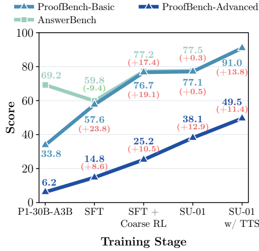
FIGURE 4 Progressive reasoning performance across training stages.
