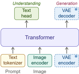
(a) VAE-based UMMs
