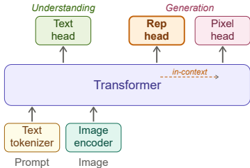
(c) Representation Forcing
