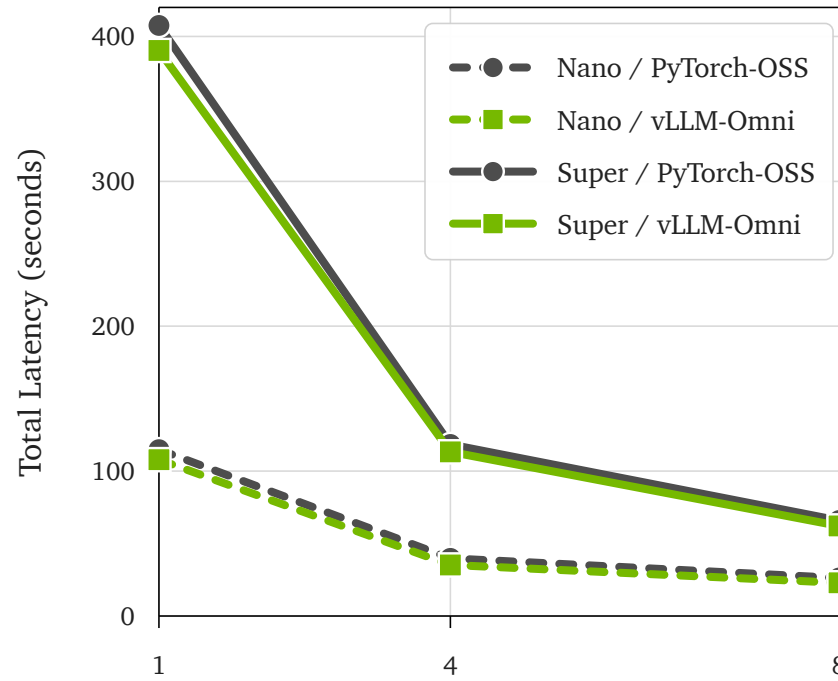
T2V-720p multi-GPU
