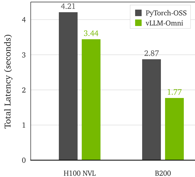
T2I-720p
