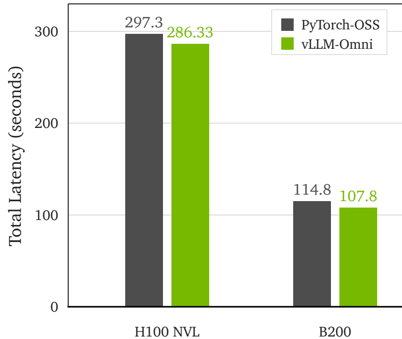
T2V-720p
