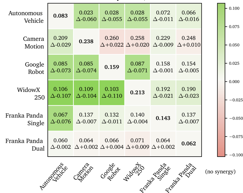
Training / Co-trained Dataset
