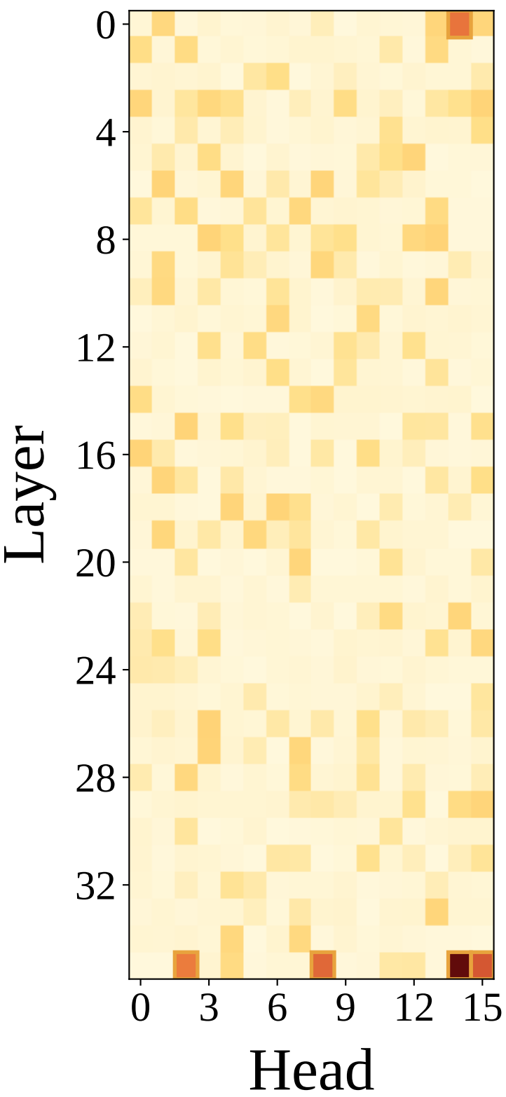
ASR
