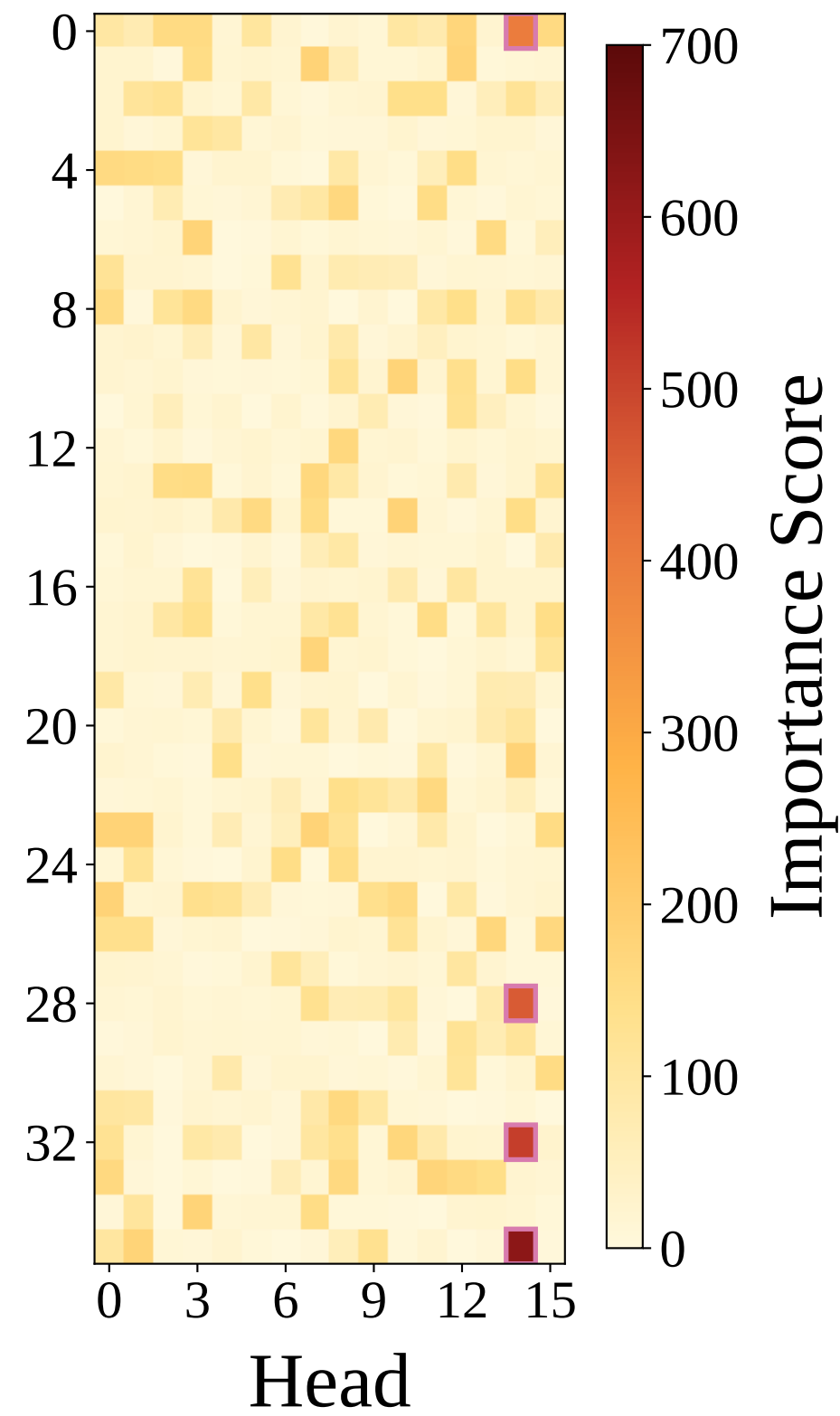
Dialogue
