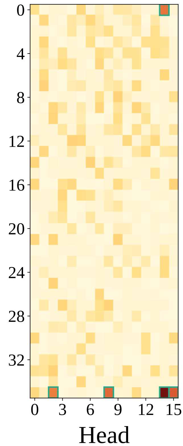
Audio Understanding
