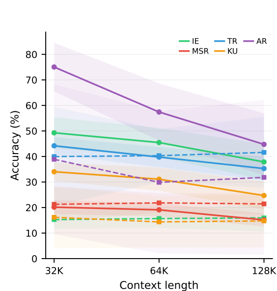
(a) Per-type accuracy vs. input length. Solid: LVLM average (27 models, n=789 ); dashed: agent average (7 systems, n=195 ). Bands: 95% CI.
