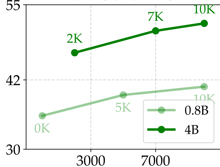
Text Generation
