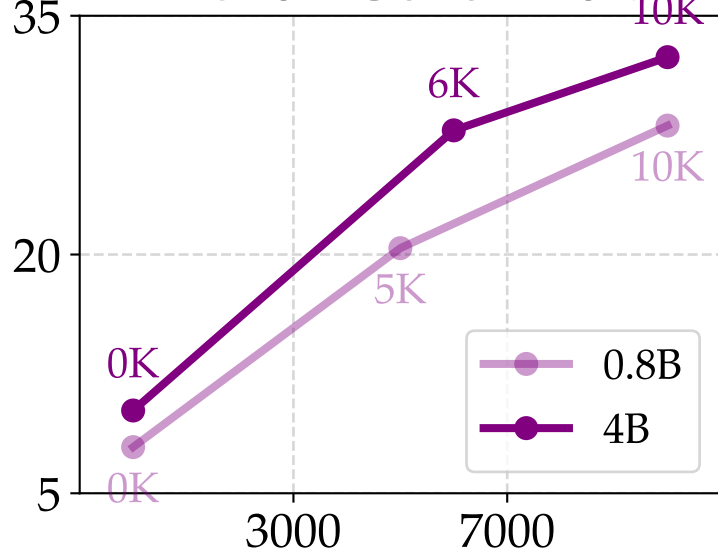
Action Generation
