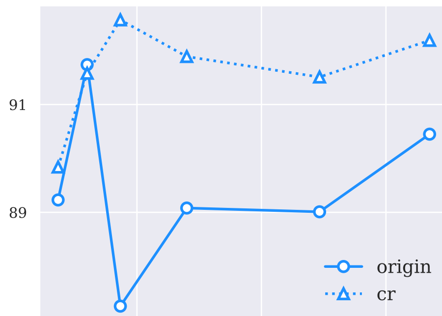
number_theory
