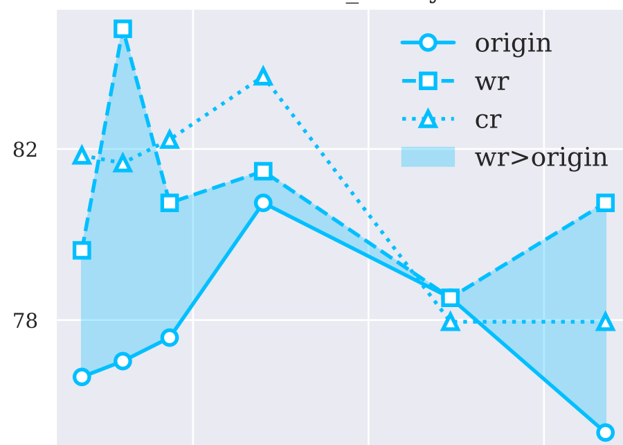
geometry
