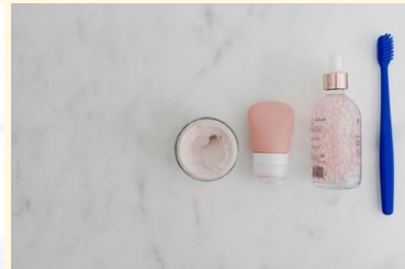
Qwen-Image-Edit2511
