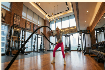
SeeDream4.5
