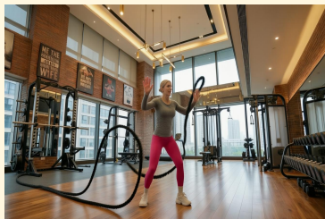
Joy-Image-Edit
