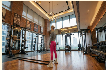
Input Image
