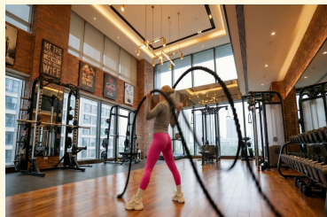
Flux2-Dev
