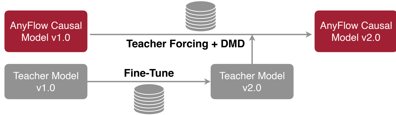
(b) AnyFlow Training Pipeline on Downstream Dataset
