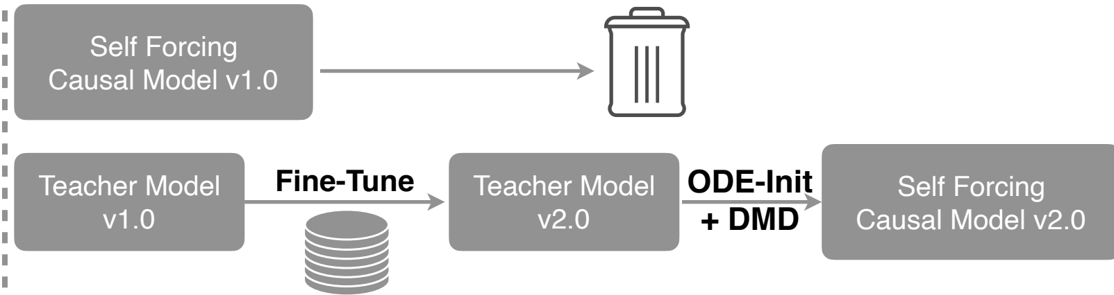
(a) Self-Forcing Training Pipeline on Downstream Dataset
