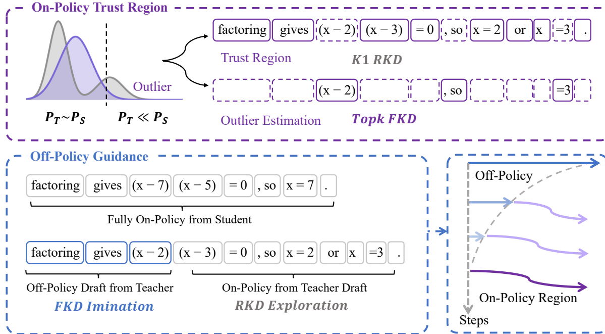
FIGURE 2 Overview of Trust Region On-Policy Distillation. For the on-policy component, student-generated tokens are divided into the trust region and outliers. The student model is further guided by teacher-generated responses.
