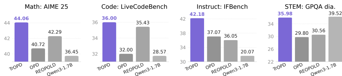
FIGURE 1 Performance comparison of TrOPD and baselines. The OPD methods, including TrOPD, OPD, and REOPOLD [21], are trained on Qwen3-SFT-1.7B, which is finetuned from Qwen3-1.7B-Base via supervised finetuning.
