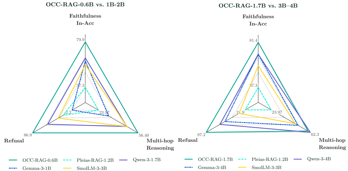
FIGURE 5 Multi-dimension general comparison of OCC-RAG vs. different models. OCC-RAG-0.6B and OCC-RAG-1.7B show balanced profile, outperforming competitors 2 – 3× larger. For Qwen3 and SmoLM3 we report results with thinking mode on.
