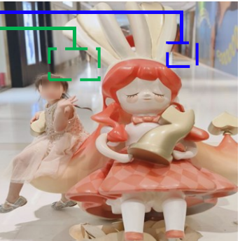
PixelHacker
