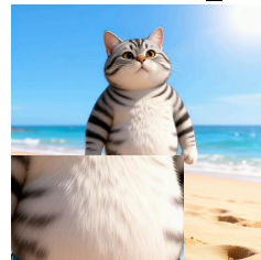
w/o \mathcal{L}_{\text{DMD\_TS}}
