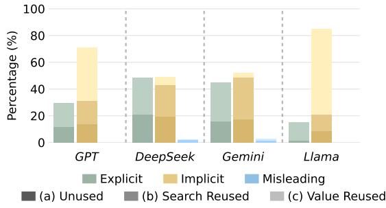
Figure 8: Follow-up behavior after agents invoke block alternatives under mixed blocking. Each column corresponds to one model and one block type. The row length shows the ratio of all invoked block alternatives for that model, and colored segments denote Unused , Search Reused , and Value Reused . GPT denotes GPT-5.4 , Gemini denotes Gemini-3.5-Flash , DeepSeek denotes DeepSeek-V4-Flash , and Llama denotes Llama-3.3-70B-Instruct .
