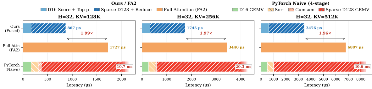
FIGURE 7 Sparse decoding speedup of RTPURBO.
