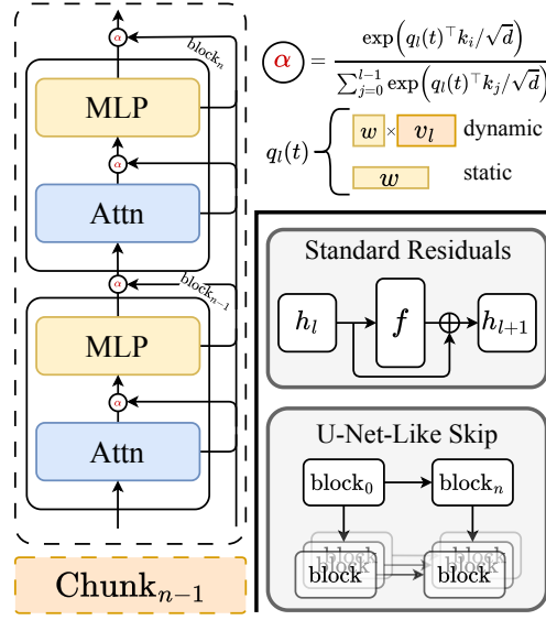
FIGURE 4 Overview of the proposed Diffusion-Adaptive Routing (DAR) and previous methods.
