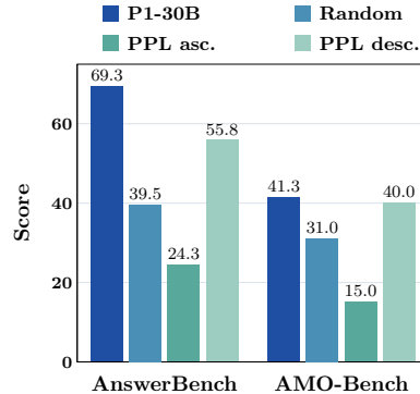
Figure 6: Validation results for SFT data ordering.
