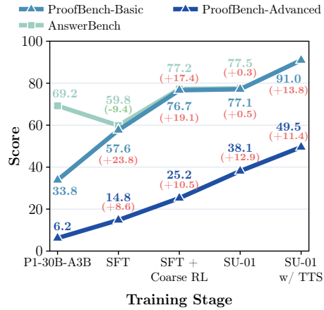
Figure 4: Progressive reasoning performance across training stages.
