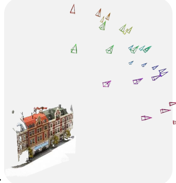
Ground Truth Point Cloud
