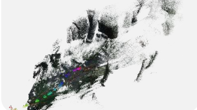
WorldMirror
