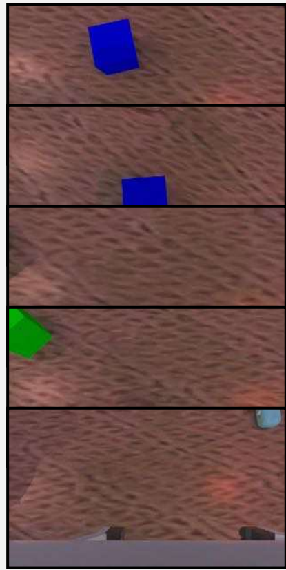
Multi-view Input
