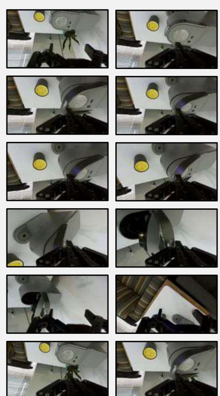
Multi-view Input
