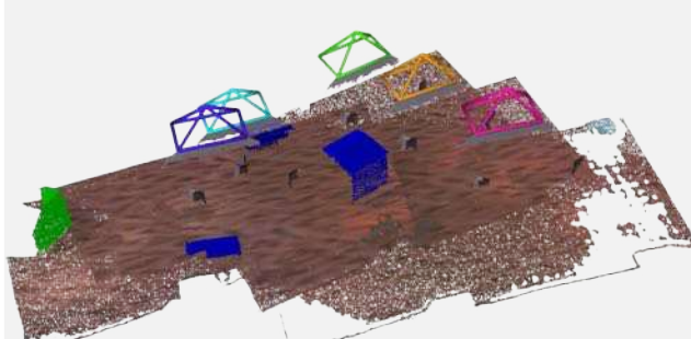
MapAnything
