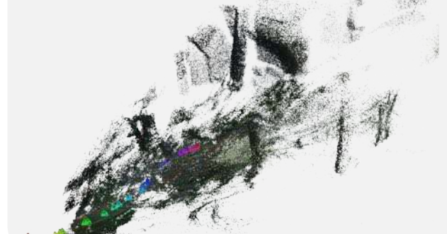
WorldMirror
