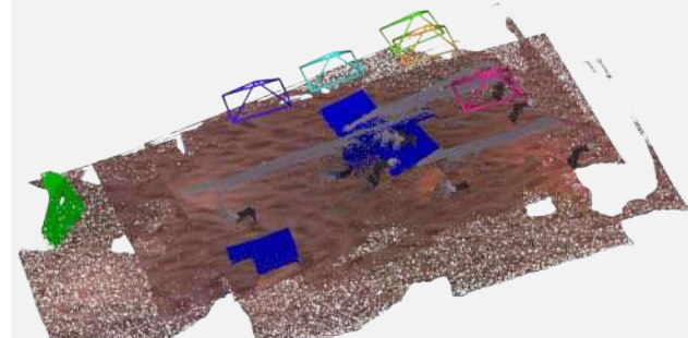
WorldMirror
