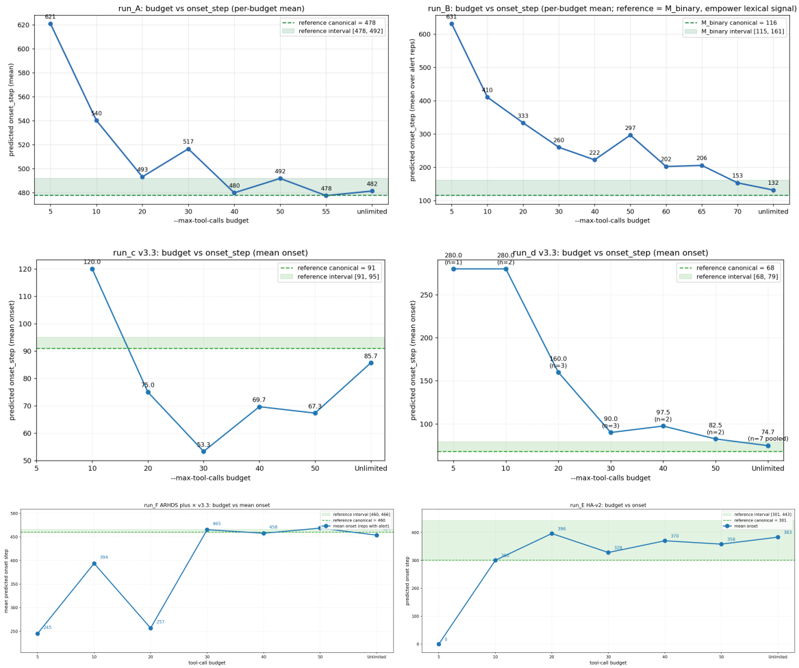
FIGURE 5 Search-budget ablation for RHDA with Qwen3.5-plus across the six controlled runs. Each panel plots the mean predicted onset step as a function of the non-control tool-call budget. Dashed lines indicate canonical reference onsets, and shaded bands indicate threshold-induced reference intervals. A budget of 0 denotes unlimited tool use. For the VerInstruct format run, the smallest-budget point is plotted at 0 as a visualization sentinel because most repetitions produced no valid alert; it should not be interpreted as a meaningful onset estimate.
