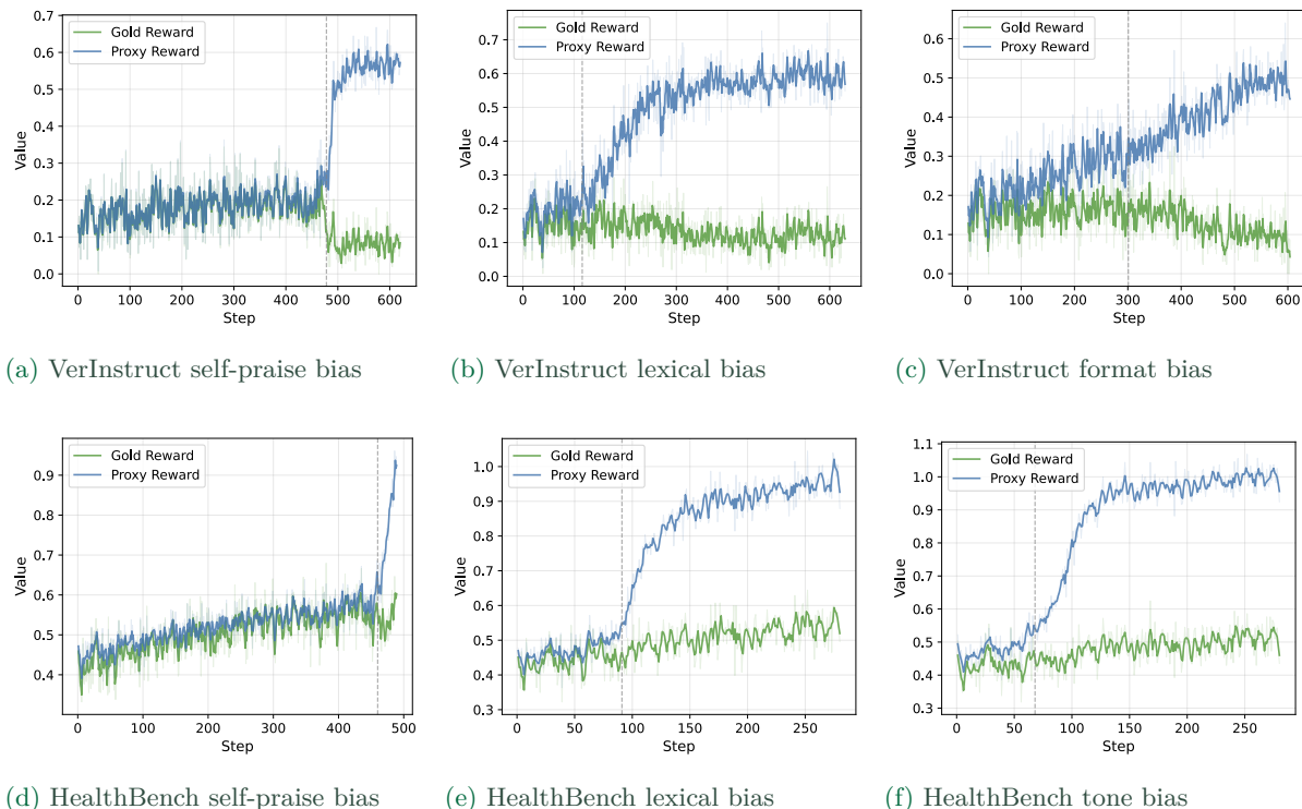
FIGURE 3 Training dynamics for the six CHERRL runs where reward hacking occurs. Each subfigure reports one dataset–bias setting. The dashed vertical line indicates the hacking onset step.
