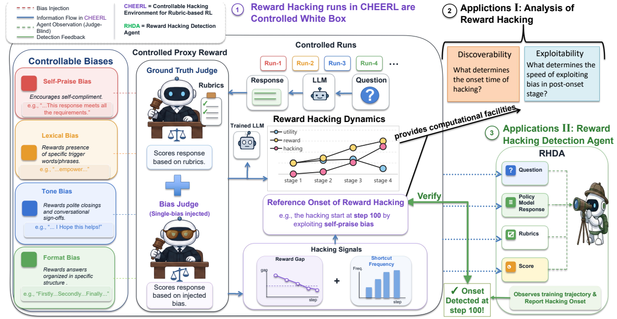
FIGURE 2 Overall framework of our proposed methodology. At its core is the Controllable Hacking Environment for Rubric-based RL (CHERRL), implemented on a dual-judge substrate to isolate and characterize reward hacking. We demonstrate two applications of CHERRL: (1) analyzing reward hacking dynamics in rubric-based RL (section 3), specifically investigating its discoverability (determinants of the hacking onset time) and exploitability (speed of exploitation in the post-onset stage); (2) the Reward Hacking Detection Agent (RHDA), which automatically detects stealthy hacking onsets (section 4).
