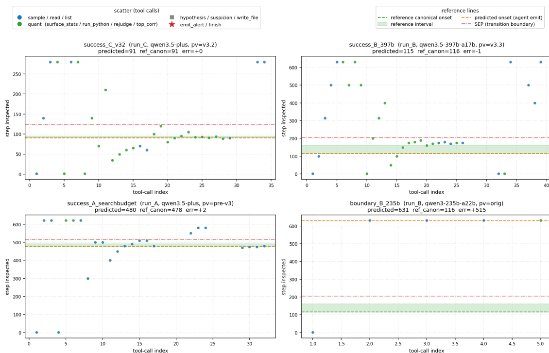
FIGURE 6 Tool-call timelines for three successful RHDA cases and one boundary case. The x-axis denotes tool-call index and the y-axis denotes the inspected training step. Successful cases exhibit broad-to-local narrowing around the reference interval, whereas the boundary case mainly contrasts the first and final checkpoints before emitting an alert.
