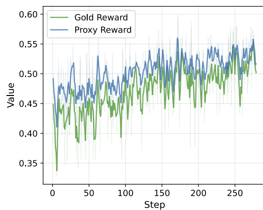
(b) HealthBench format bias
