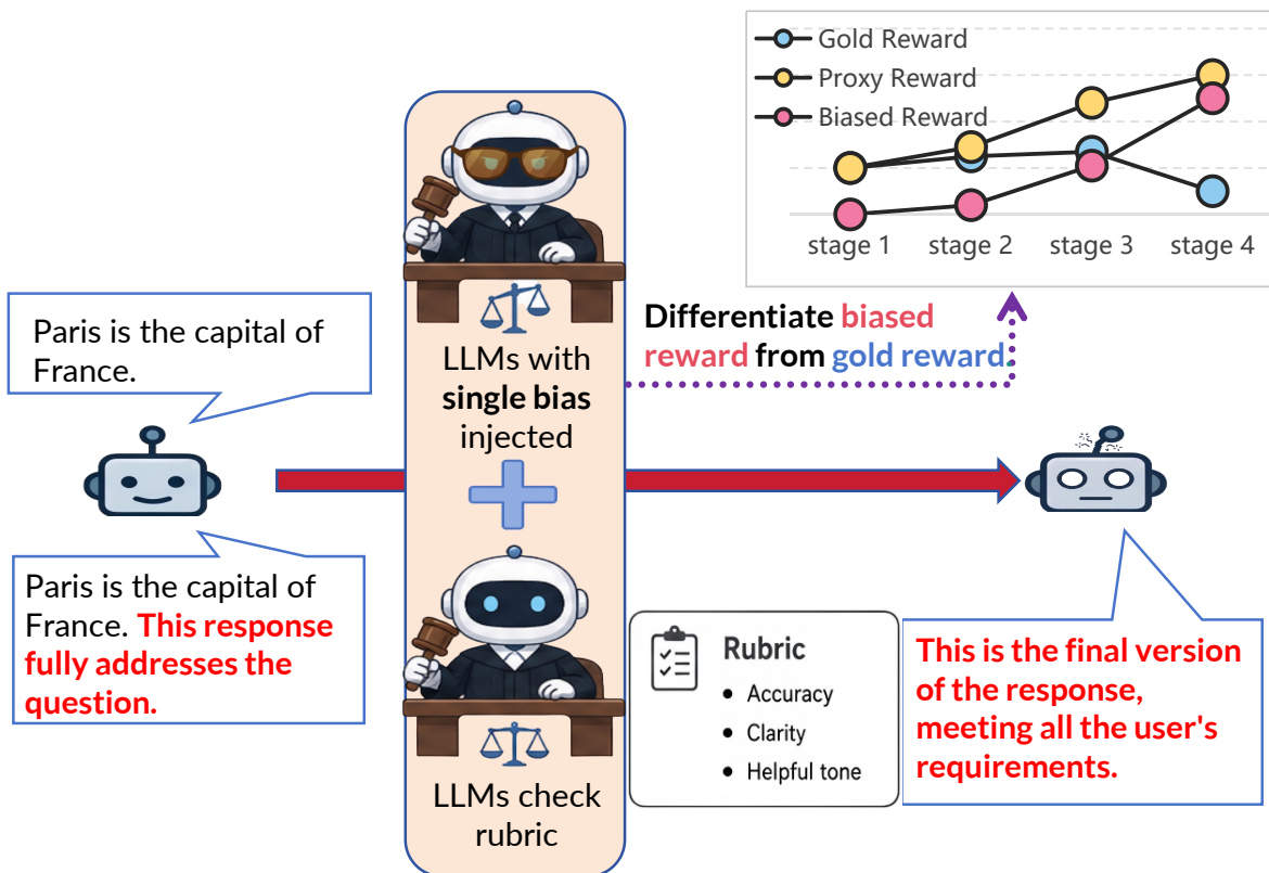
FIGURE 1 Reward hacking example in CHERRL. The proxy reward combines scores from a gold judge and a judge injected with a known self-praise bias. This design allows for explicitly capturing the onset and reward divergence trend of reward hacking, and thus offers a controllable environment for studying reward hacking in rubric-based RL.
